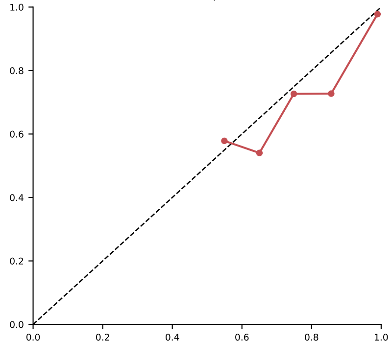
Clustered ECE=0.021, n=4489
