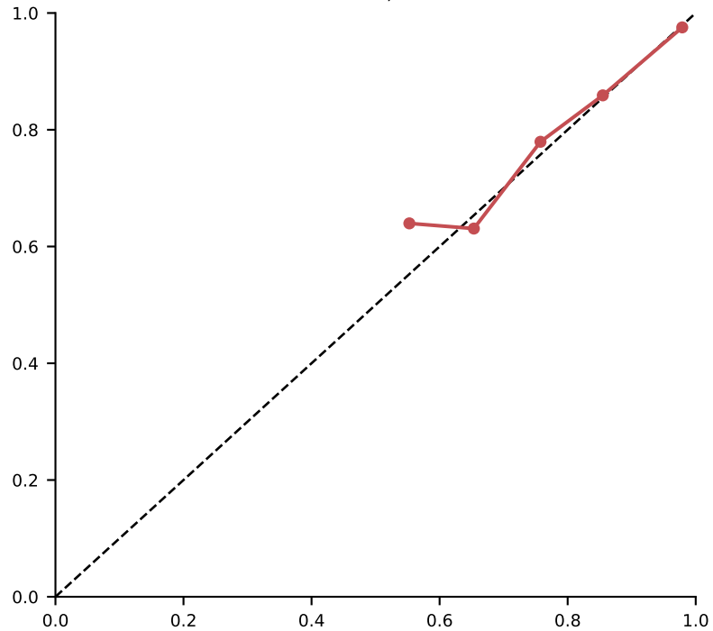
Unclustered ECE=0.007, n=3661
